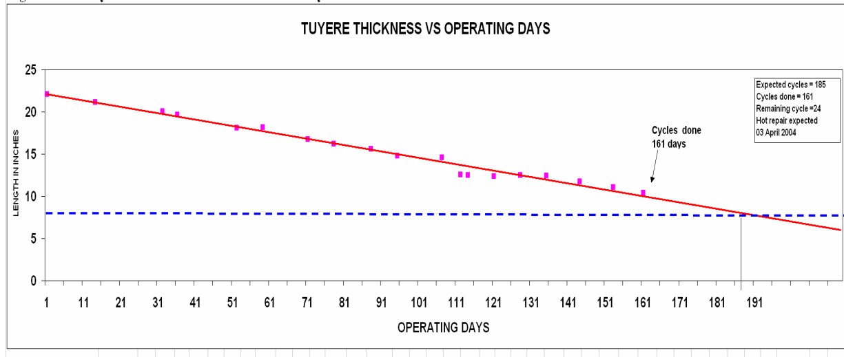
Figure 5: CT Tuyere line Measurements and Refractory Performance
