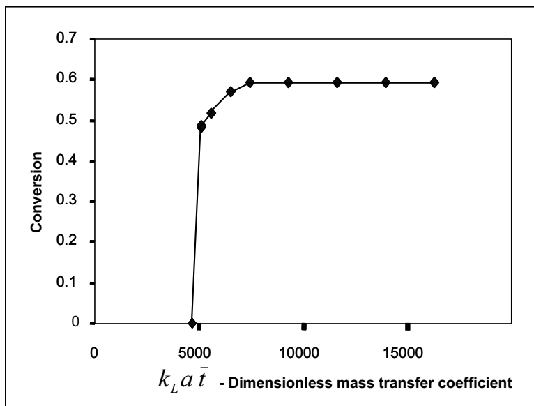
Figure 8: The effect of the mass transfer coefficient on the performance of a leaching reactor.
