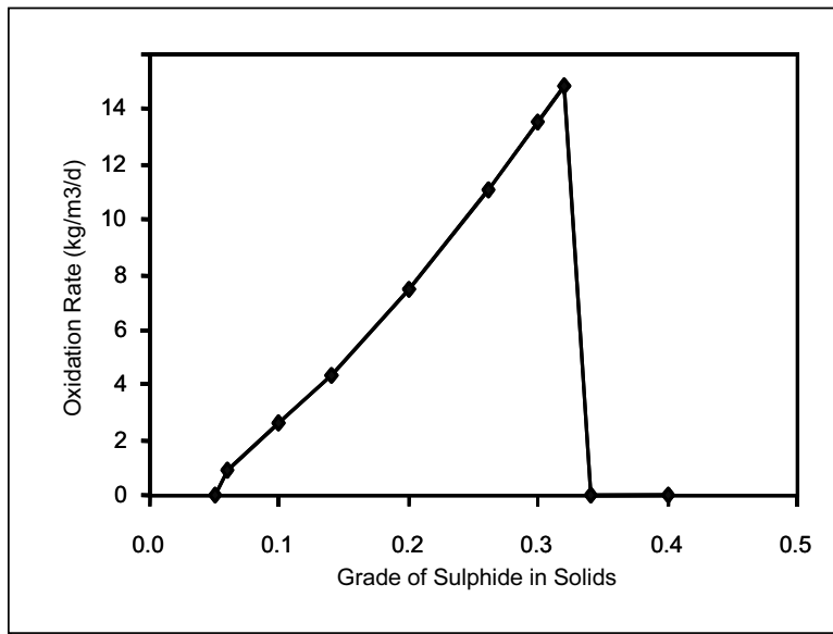
Figure 9: The effect of increasing the sulphide load on the performance of a leaching reactor.
