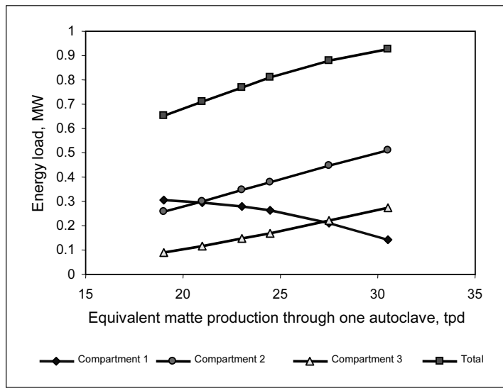
Figure 7: The energy load for heat removal from the Second Stage leach as a function of the amount of material processed in the reactor.
