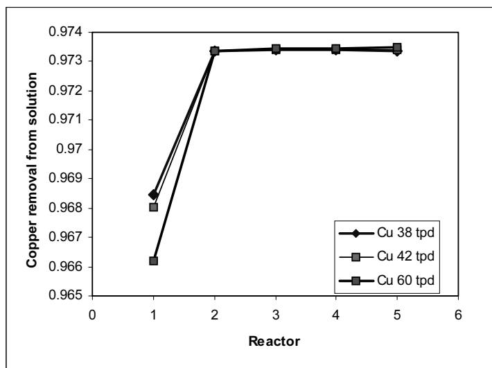
Figure 4. Effect of increases in capacity on the copper removal from solution.
