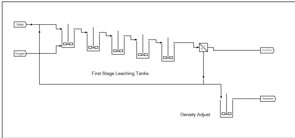
Figure2: Nickel atmospheric leach
