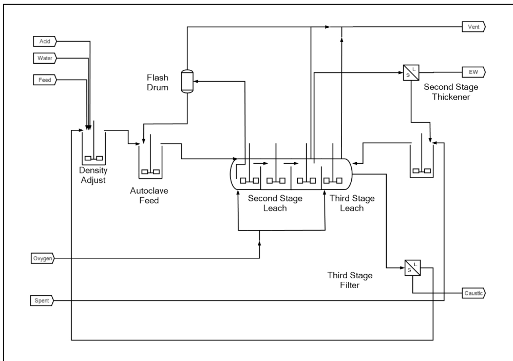
Figure 5: Second and third stage autoclave configuration.
