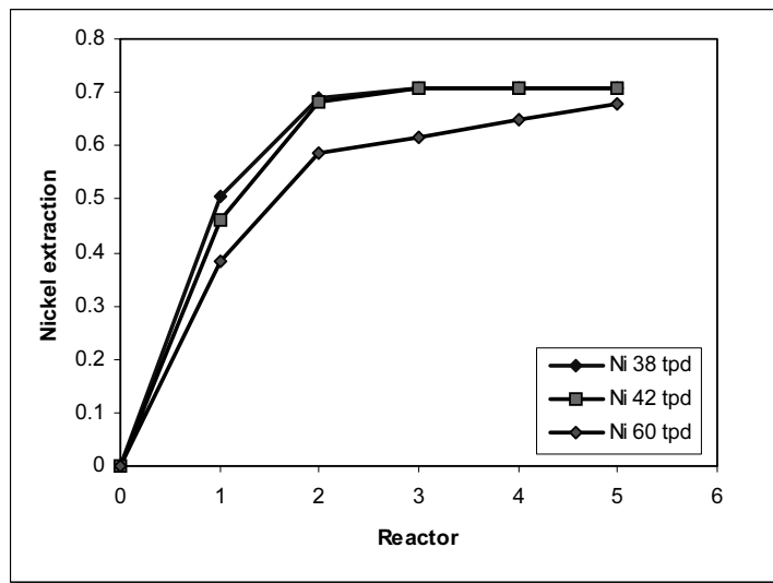
Figure 3. Nickel extraction as a function of capacity.
