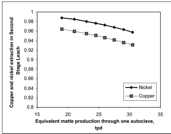
Figure 6: The copper and nickel extractions in the Second Stage leach assuming no limitations due to gas-liquid mass transfer or heat transfer.
