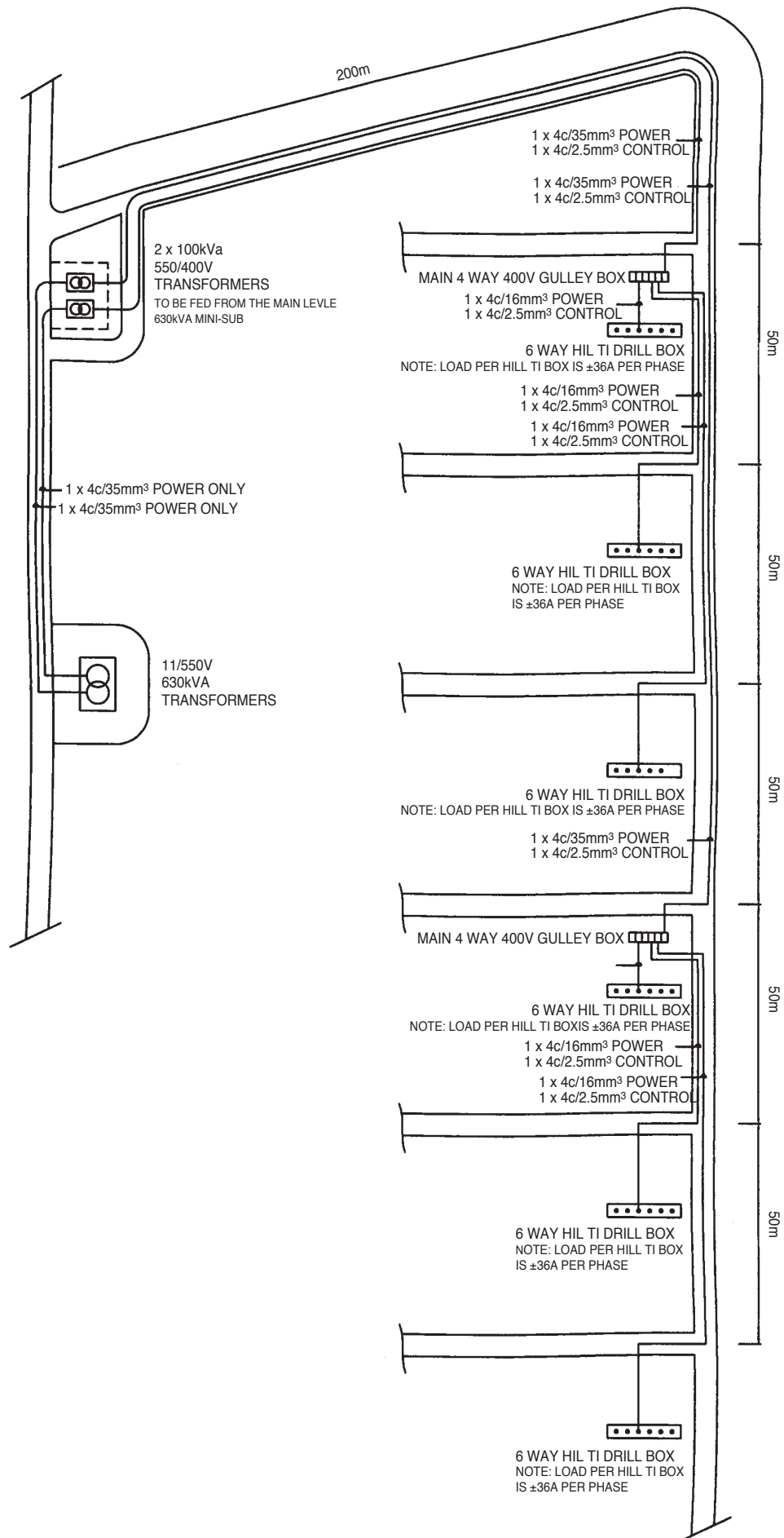
Figure 3. Single line diagram (SLD): layout of three-phase reticulation 8
