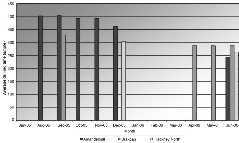
Figure 2. Average drilling cycle time in UG2 reef
