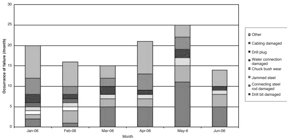
Figure 4. Modes and quantification of failures
