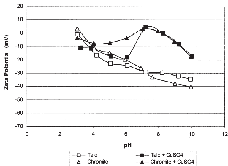
Figure 2. The effect of 10^{-4} M copper sulphate addition on the zeta potential values of talc and chromite with 10^{-3} M of potassium nitrate as indifferent electrolyte at pH of 3 to 10
