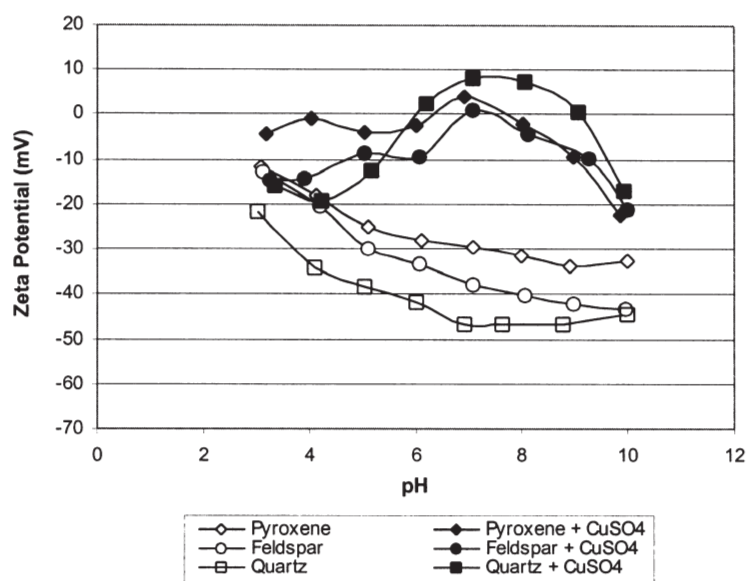
Figure 1. The effect of 10 -4 M copper sulphate addition on the zeta potential values of pyroxene, feldspar and quartz with 10 -3 M of potassium nitrate as indifferent electrolyte at pH of 3 to 10
