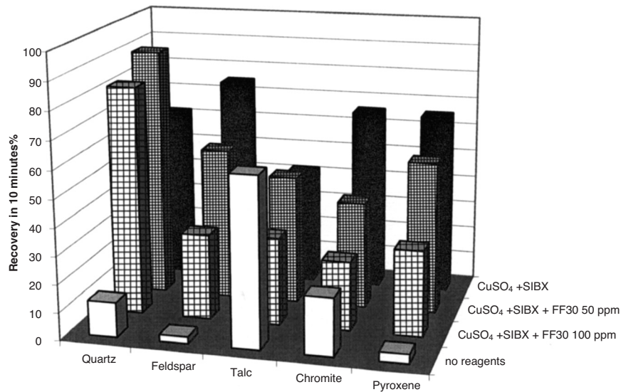
Figure 6. The effect of adding reagents with CMC (FF30) as a depressant on the floatability of quartz, feldspar, talc, chromite and pyroxene (as mass recovery percentage)
