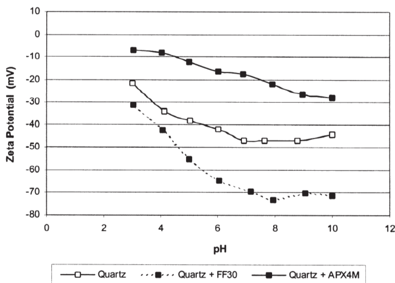
Figure 4. The effect of polymeric depressants on the zeta potential values for quartz with 10^{-3} M of potassium nitrate as an indifferent electrolyte
