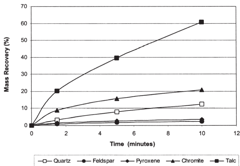
Figure 5. Natural floatability of all selected gangue minerals under 10^{-2} calcium nitrate ionic strength
