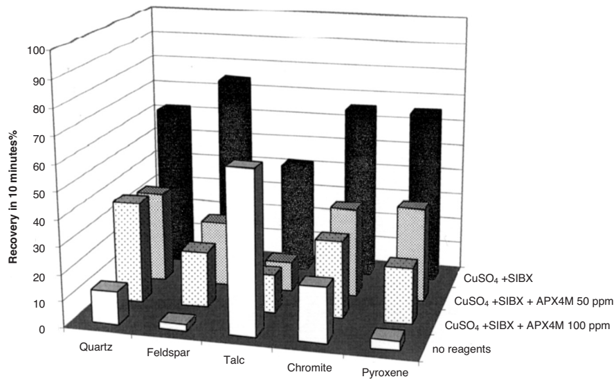
Figure 7. The effect of adding reagents with guar gum (APX4M) as a depressant on the floatability of quartz, feldspar, talc, chromite and pyroxene (as mass recovery percentage)
