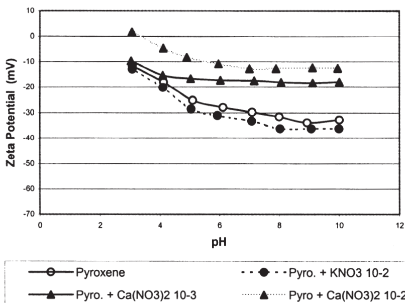
Figure 3. The effect of calcium ions and different ionic strength ( 10^{-3} ; 10^{-2} ) on the zeta potential values of pyroxene
