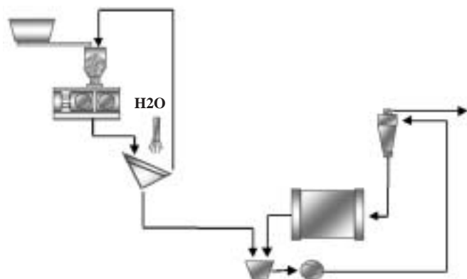
Figure 4. HPGR in closed circuit mode with a ball mill
