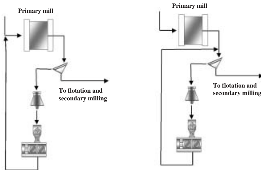
Figure 6. AG/SAG circuit with high pressure grinding rolls for pebble crushing
