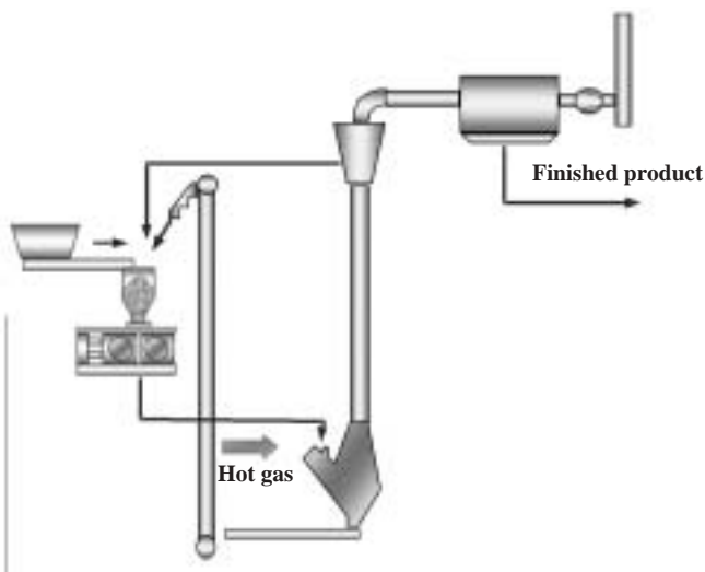
Figure 9. HPGR in dry grinding mode
