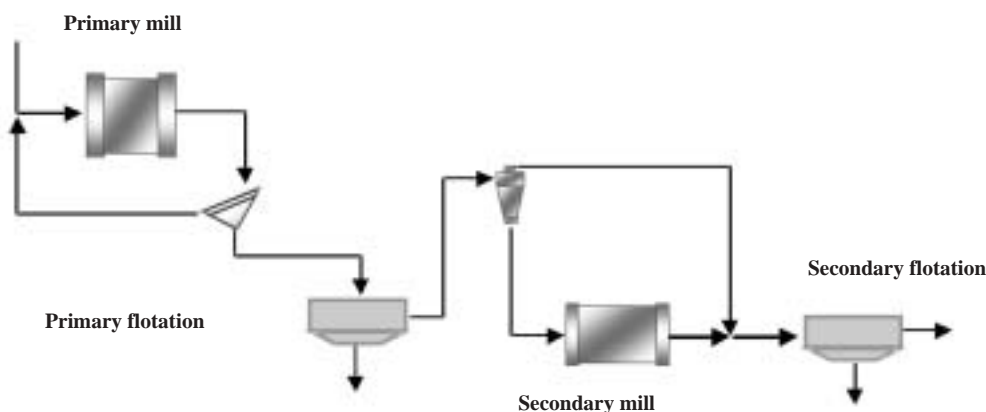
Figure 5. Typical flow sheet for a milling plant in the platinum industry
