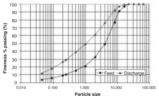
Figure 2. Expected size distribution for an industrial unit
