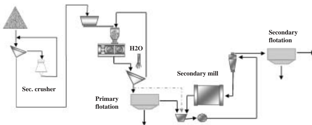
Figure 7. HPGR in closed circuit 'wet mode' (separating HPGR from the crushing circuit and combining it with the ball mill grinding plant)
