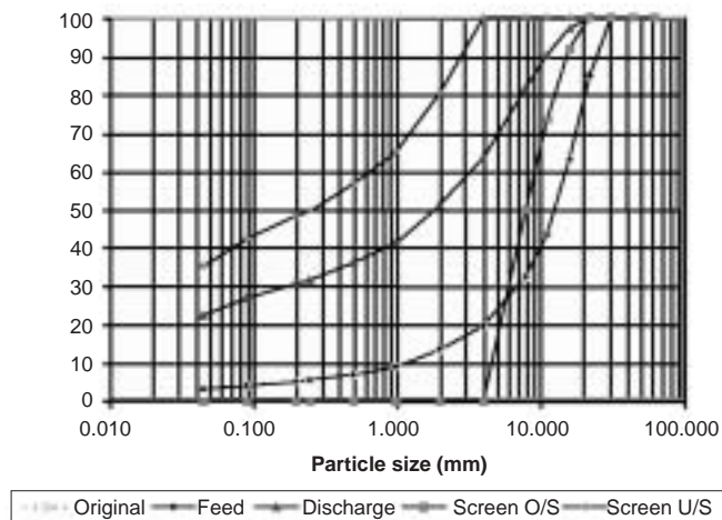
Figure 3. Size distribution for UG2 ore
