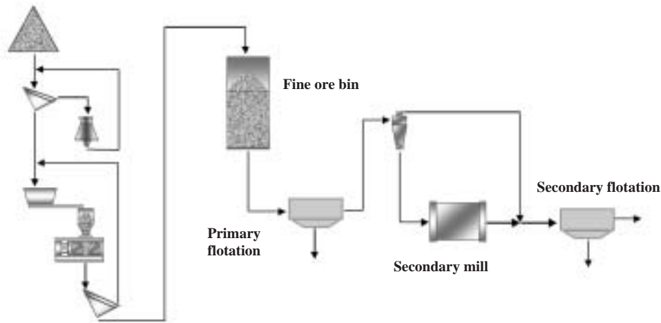
Figure 8. HPGR in closed circuit—'dry mode'
