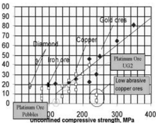
Figure 1—ATWAL wear index for various ores
