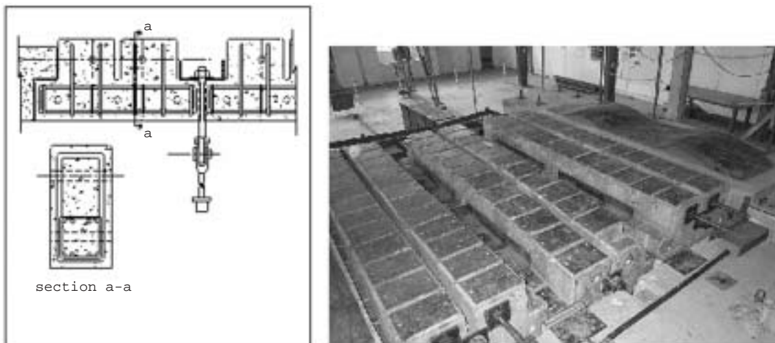
Figure 3. Detail of concrete blocks and tie-down cables with accompanying photograph of the three Voussoir beams
