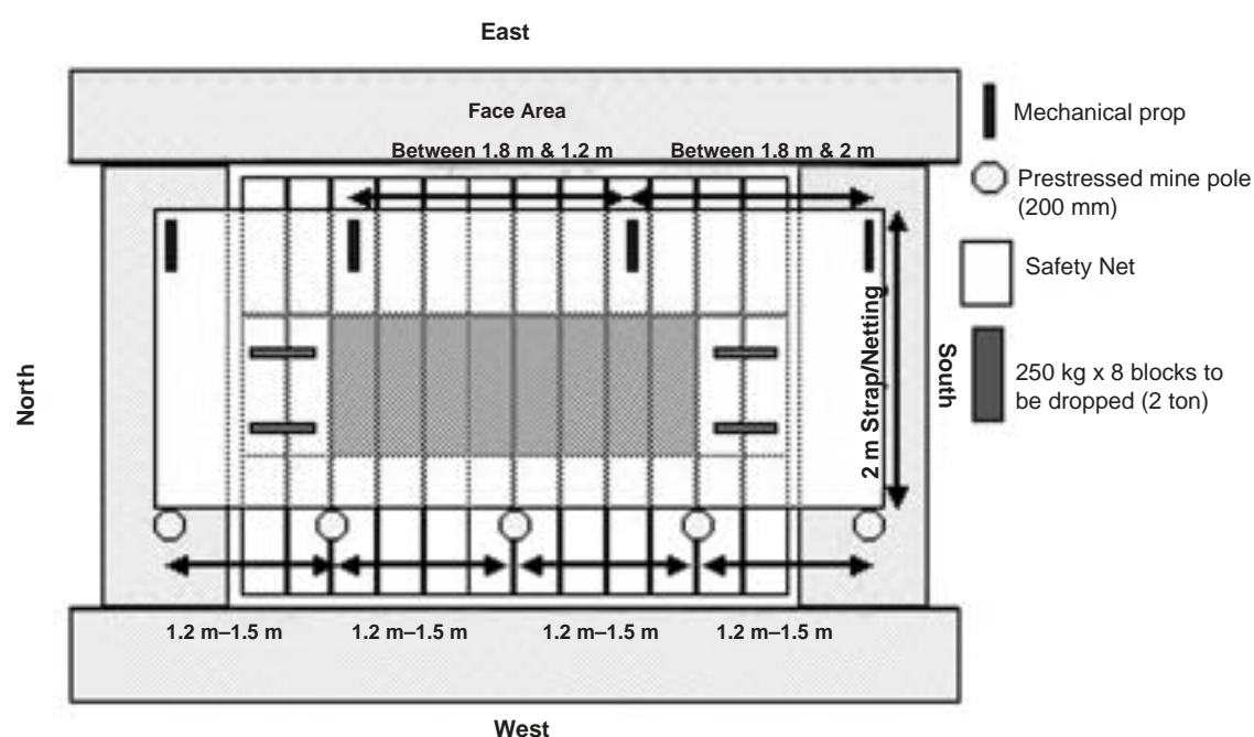
Figure 4. Plan view of a typical fall of ground test configuration with eight blocks weighting 2 tons total free to fall onto the safety net
