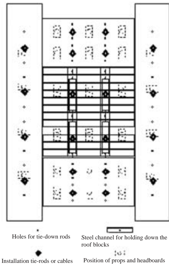
Figure 2. Plan view of the testing facility
