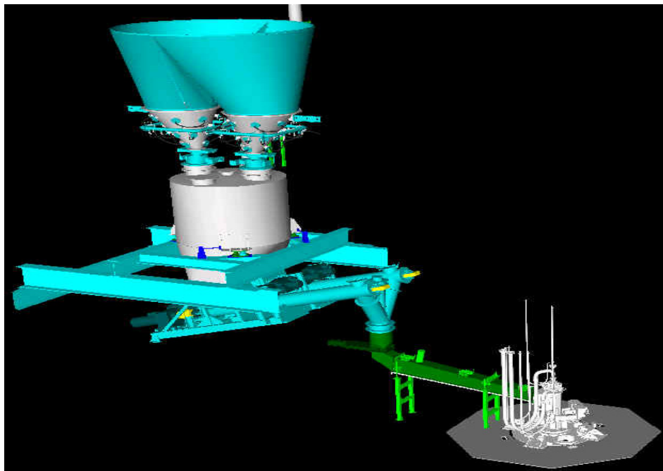
Figure 11. Proposed feed arrangement
